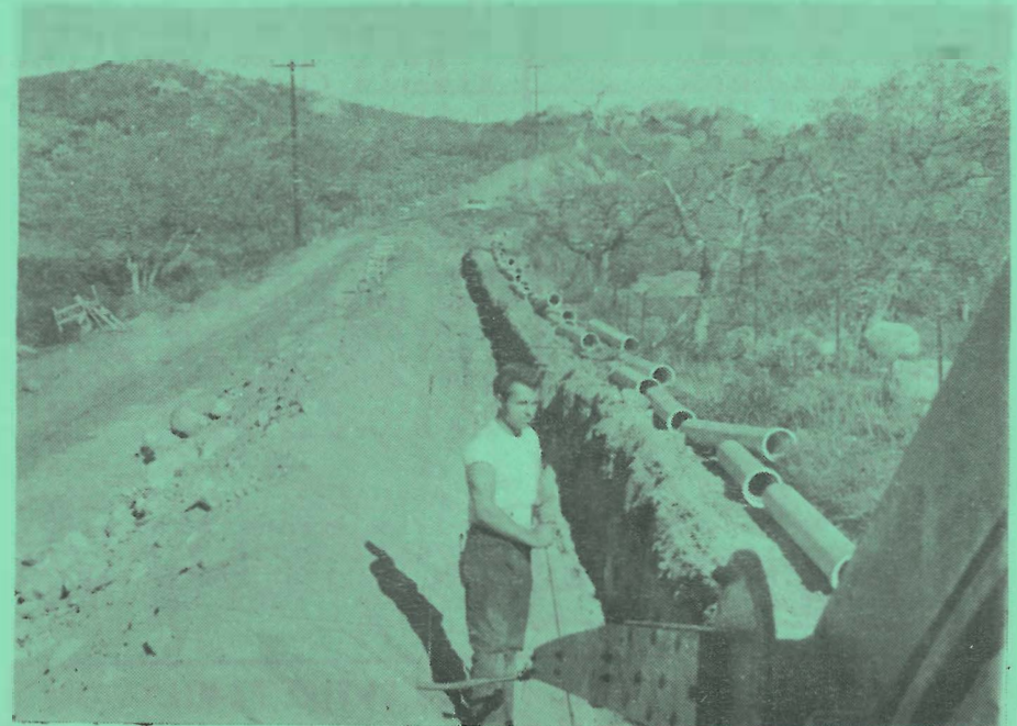
MOST THRILLING SCENE THIS WEEK WAS LAYING OF 10 INCH WATER MAIN DOWN SOUTH GRADE ROAD TO PIERCE SUBDIVISION, VIEJAS VIEW RANCH. HFRE HAMM BROS. DIGGER IS SHOWN WITH OILER
